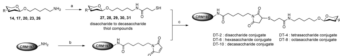
Scheme 3. Oligosaccharide conjugation to the carrier protein. Reagents and conditions: a) DTSSP, PBS buffer (pH 7.4), RT; DTT, 40°C, 70–75%; b) sulfo-EMCS, PBS buffer (pH 8.0), RT; c) PBS buffer (pH 7.4), RT.
