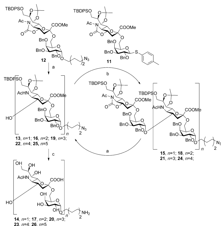
Scheme 2. Synthesis of oligosaccharides. Reagents and conditions: a) NaOMe, MeOH, RT, 65–75%; b) NIS, TFOH, CH 2 Cl 2 , –40°C, 64% for 15 , 52% for 18 , 46% for 21 , 35% for 24 ; c) BF 3 ·OEt 2 , acetonitrile, 0°C; NaOH, MeOH/H 2 O; Pd(OH) 2 /H 2 , MeOH/H 2 O, 35–50%, over three steps. NIS = N -iodosuccinimide.
