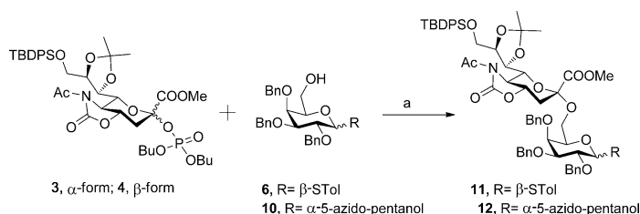
Scheme 1. Synthesis of disaccharide building blocks 11 and 12 . Reagents and conditions: a) TMSOTf, CH 2 Cl 2 , –70°C, about 90%. TMSOTf = tri-methylsilyl trifluoromethanesulfonate.
